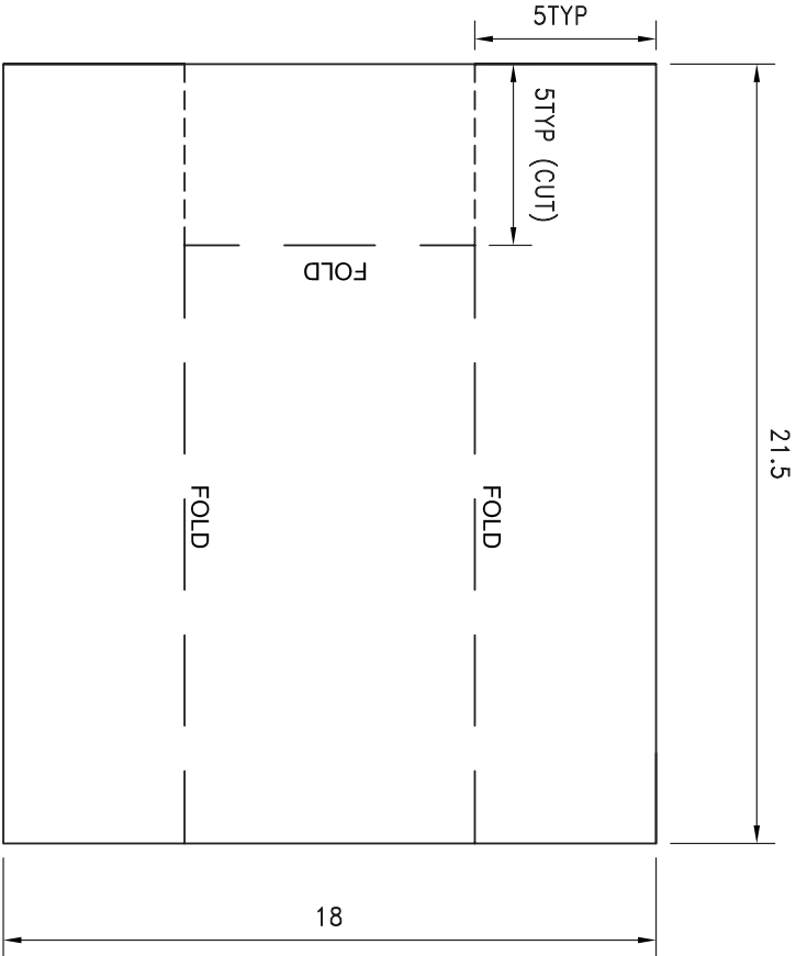
PLAN VIEW 1 LKG DOWN DECK INSTALLATION
